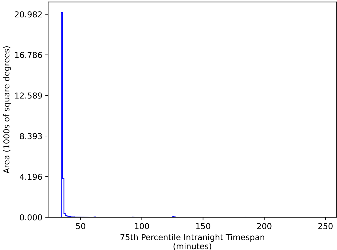
weather_cloudso0v3.4_10yrs All sky gr bands: 75th Percentile Intranight Timespan
