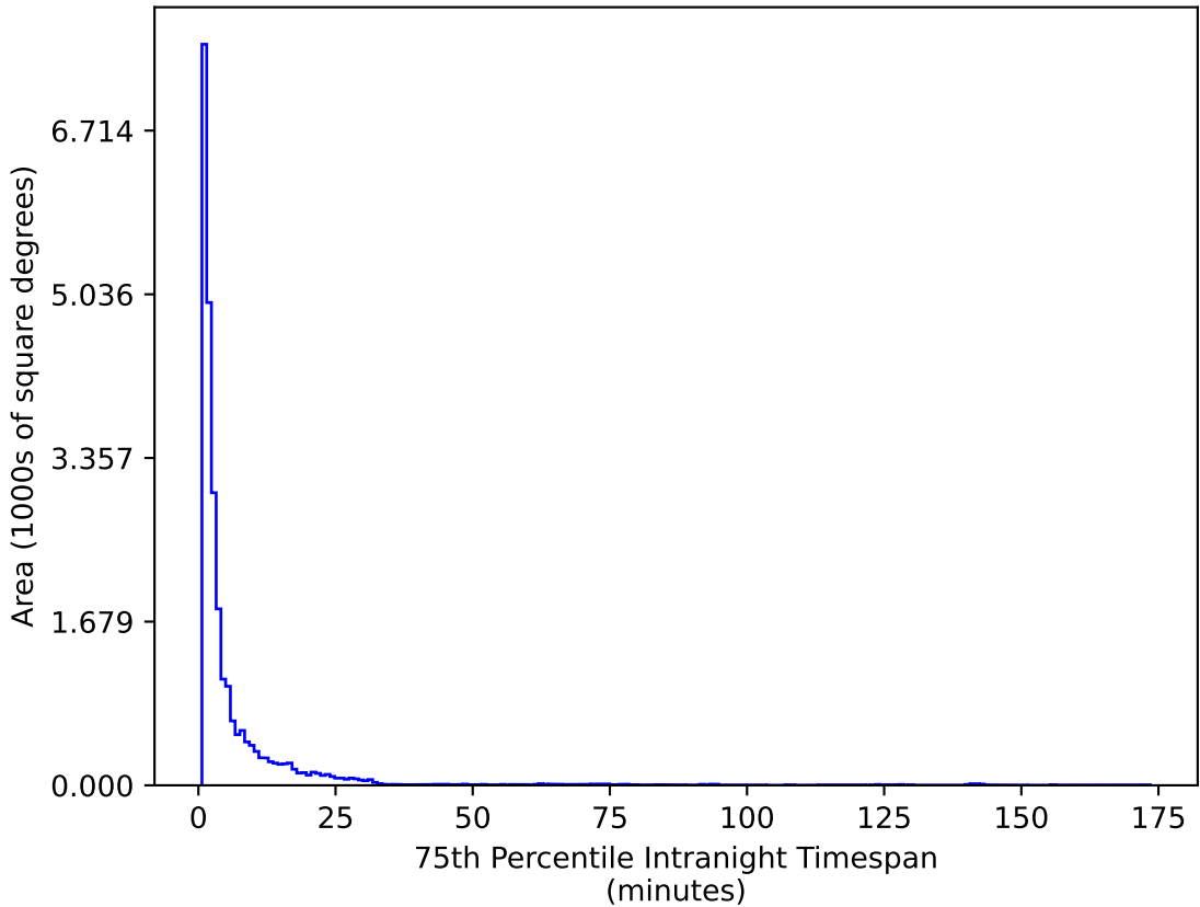
weather_cloudso0v3.4_10yrs All sky g band: 75th Percentile Intranight Timespan
