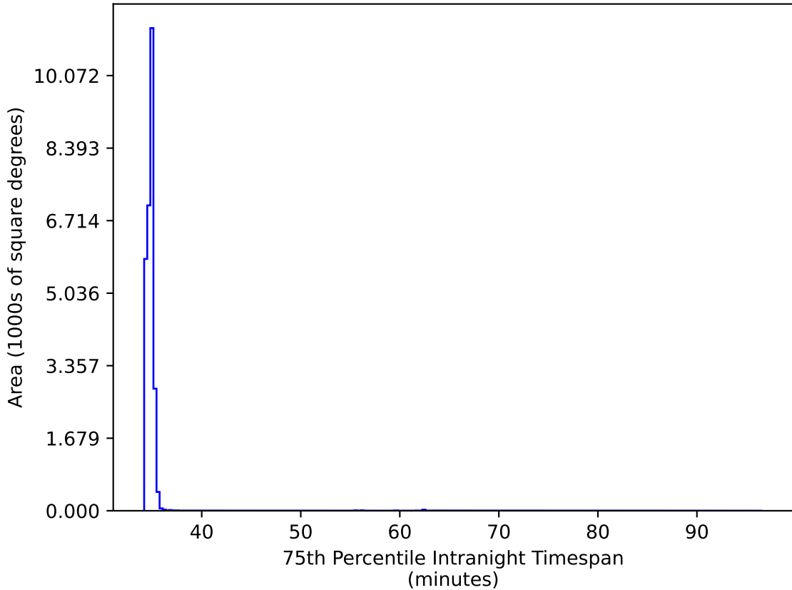
weather_cloudso0v3.4_10yrs All sky: 75th Percentile Intranight Timespan
