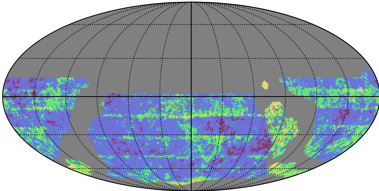
weather_cloudso0v3.4_10yrs WFD z band: 20thPercentile Inter-Night Gap
