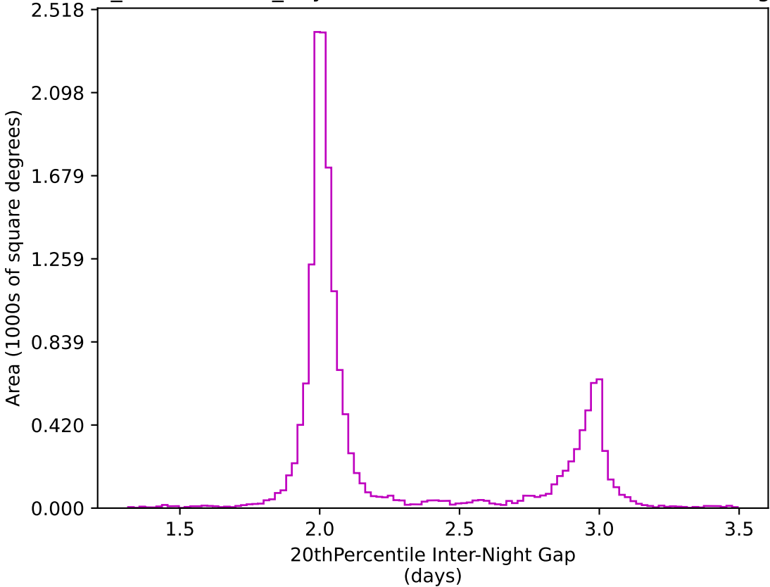
weather_cloudso0v3.4_10yrs WFD z band: 20thPercentile Inter-Night Gap
