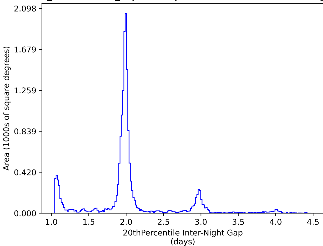
weather_cloudso0v3.4_10yrs WFD y band: 20thPercentile Inter-Night Gap
