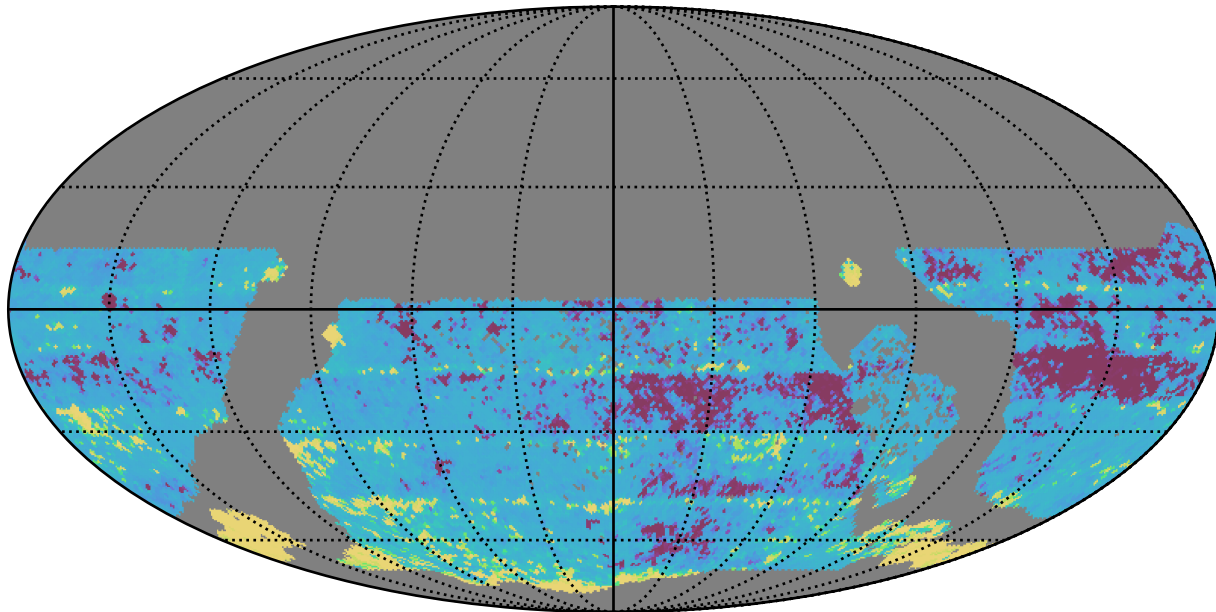
weather_cloudso0v3.4_10yrs WFD r band: 20thPercentile Inter-Night Gap
