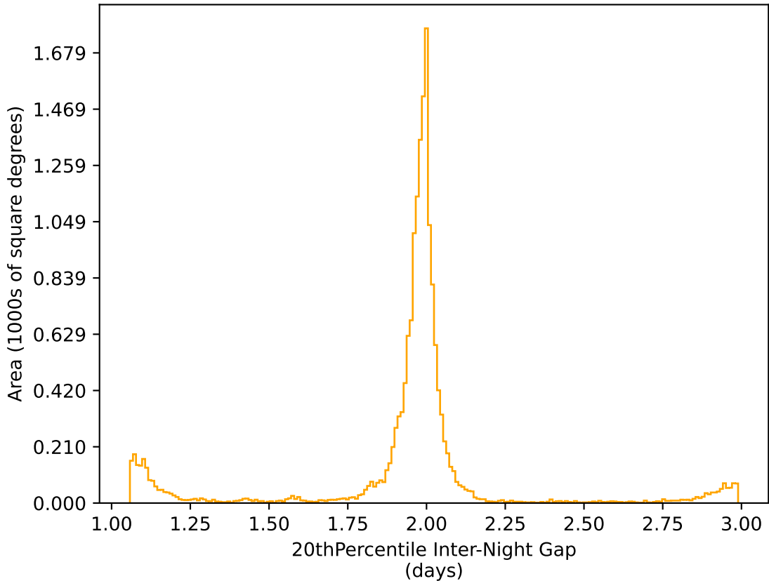
weather_cloudso0v3.4_10yrs WFD r band: 20thPercentile Inter-Night Gap
