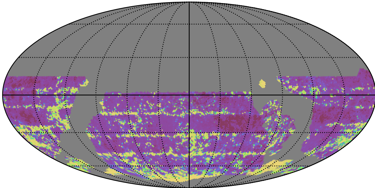
weather_cloudso0v3.4_10yrs WFD i band: 20thPercentile Inter-Night Gap
