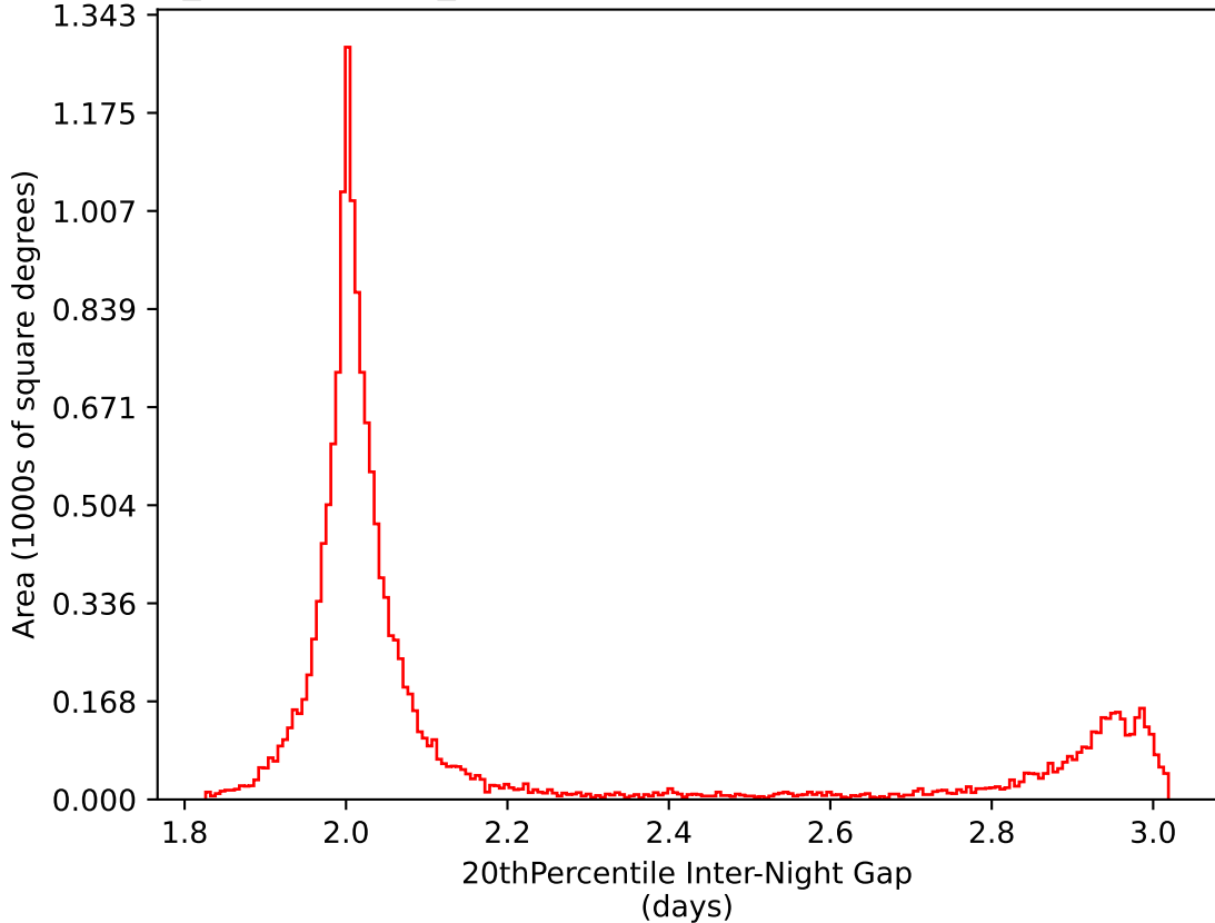
weather_cloudso0v3.4_10yrs WFD i band: 20thPercentile Inter-Night Gap
