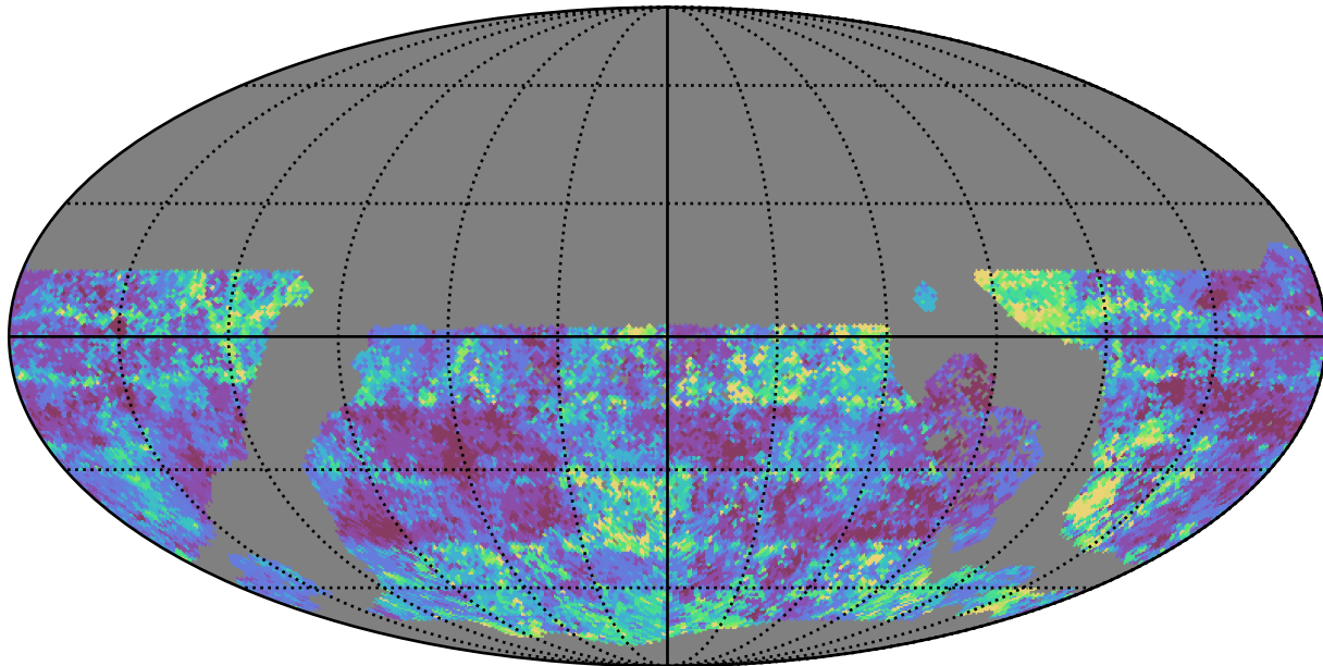
weather_cloudso0v3.4_10yrs WFD g band: 20thPercentile Inter-Night Gap
