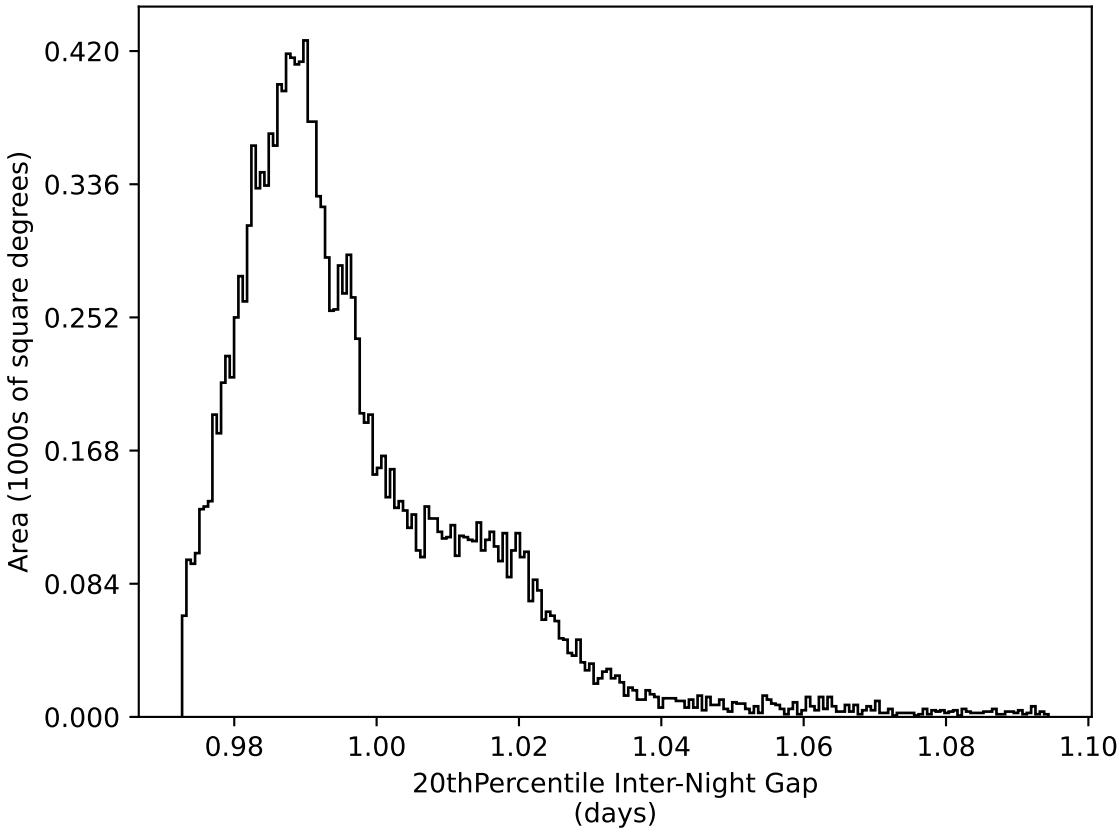
weather_cloudso0v3.4_10yrs WFD all bands: 20thPercentile Inter-Night Gap
