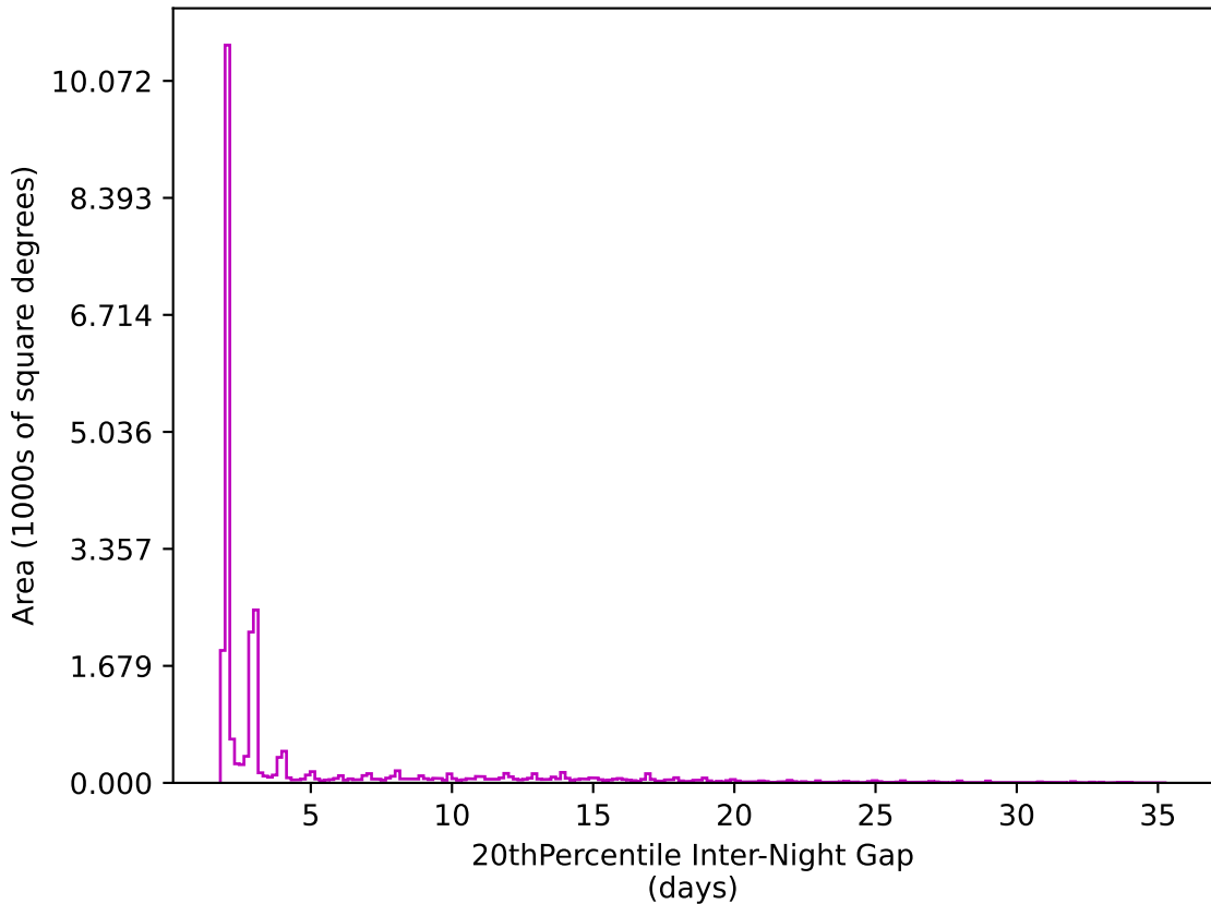
weather_cloudso0v3.4_10yrs All sky z band: 20thPercentile Inter-Night Gap
