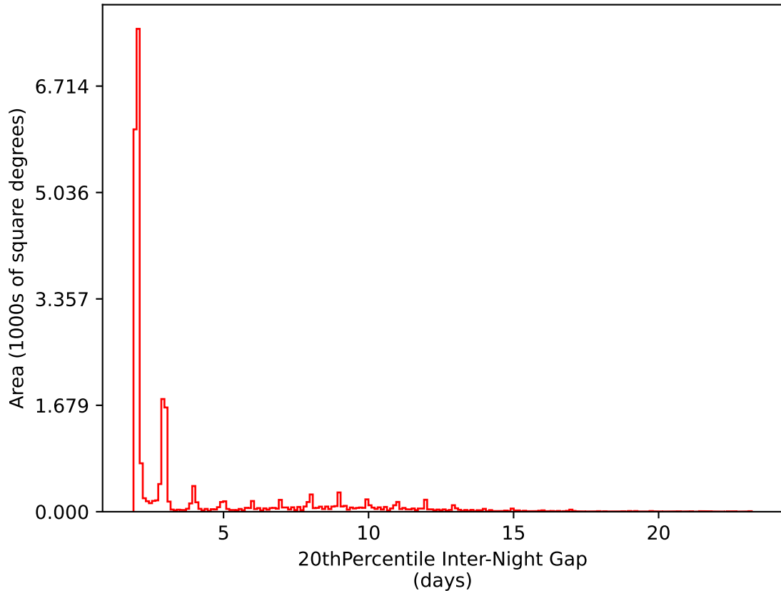
weather_cloudso0v3.4_10yrs All sky i band: 20thPercentile Inter-Night Gap
