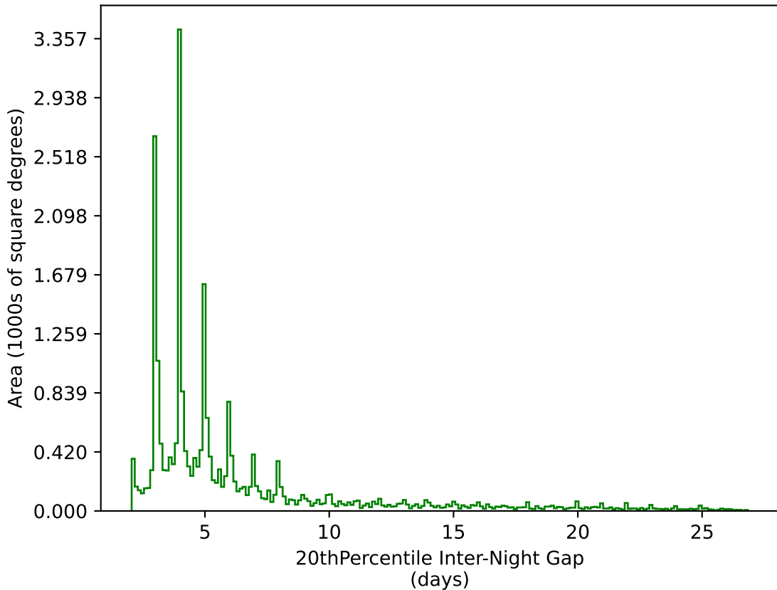
weather_cloudso0v3.4_10yrs All sky g band: 20thPercentile Inter-Night Gap
