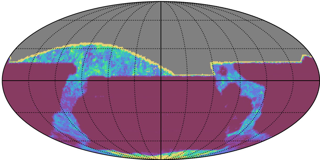
weather_cloudso0v3.4_10yrs All sky all bands: 20thPercentile Inter-Night Gap
