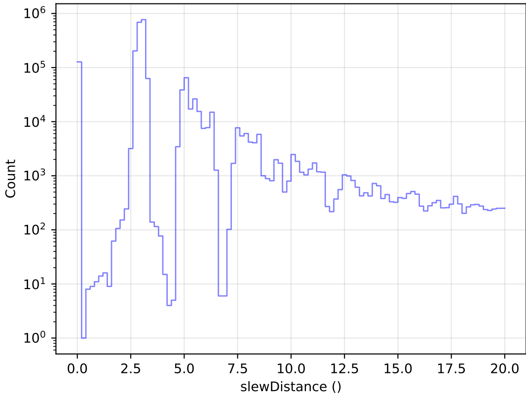
weather_cloudso0v3.4_10yrs All visits: Zoom Slew Distance Histogram
