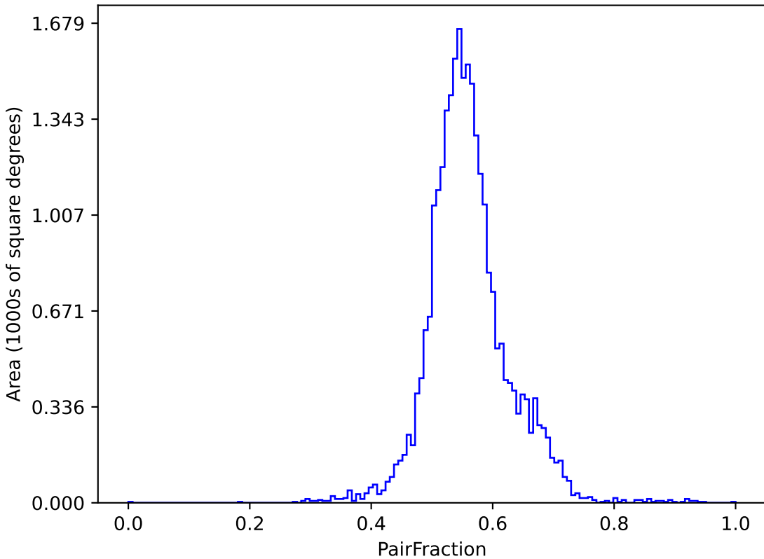
weather_cloudso0v3.4_10yrs (g or r or i): PairFraction
