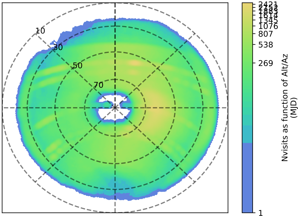
weather_cloudso0v3.4_10yrs z: Nvisits as function of Alt/Az
