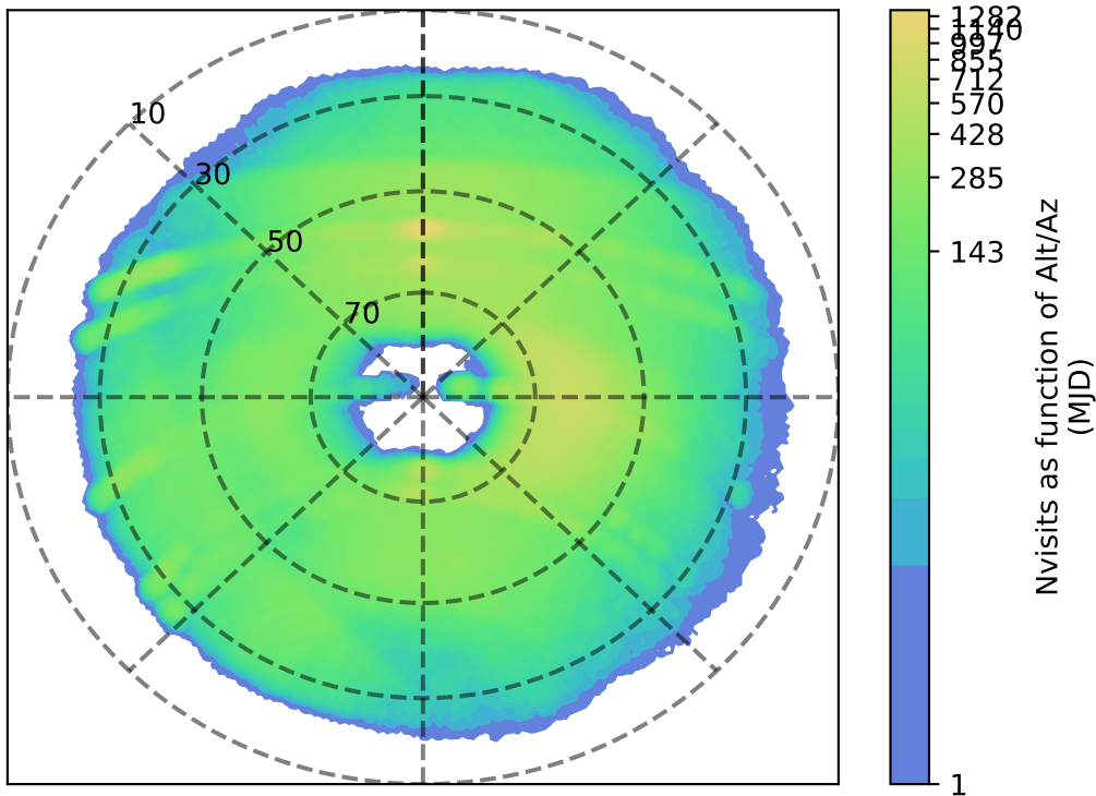
weather_cloudso0v3.4_10yrs g: Nvisits as function of Alt/Az
