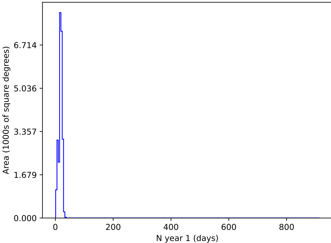
weather_cloudso0v3.4_10yrs y and night < 365: N year 1
