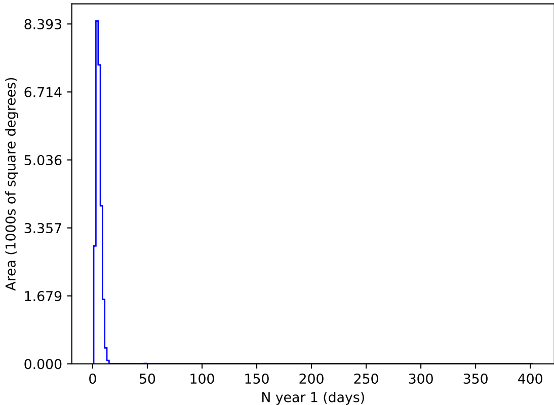
weather_cloudso0v3.4_10yrs u and night < 365: N year 1
