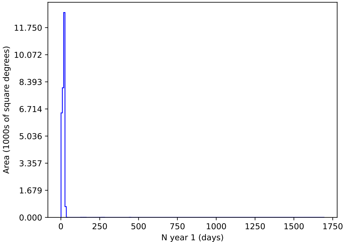
weather_cloudso0v3.4_10yrs r and night < 365: N year 1
