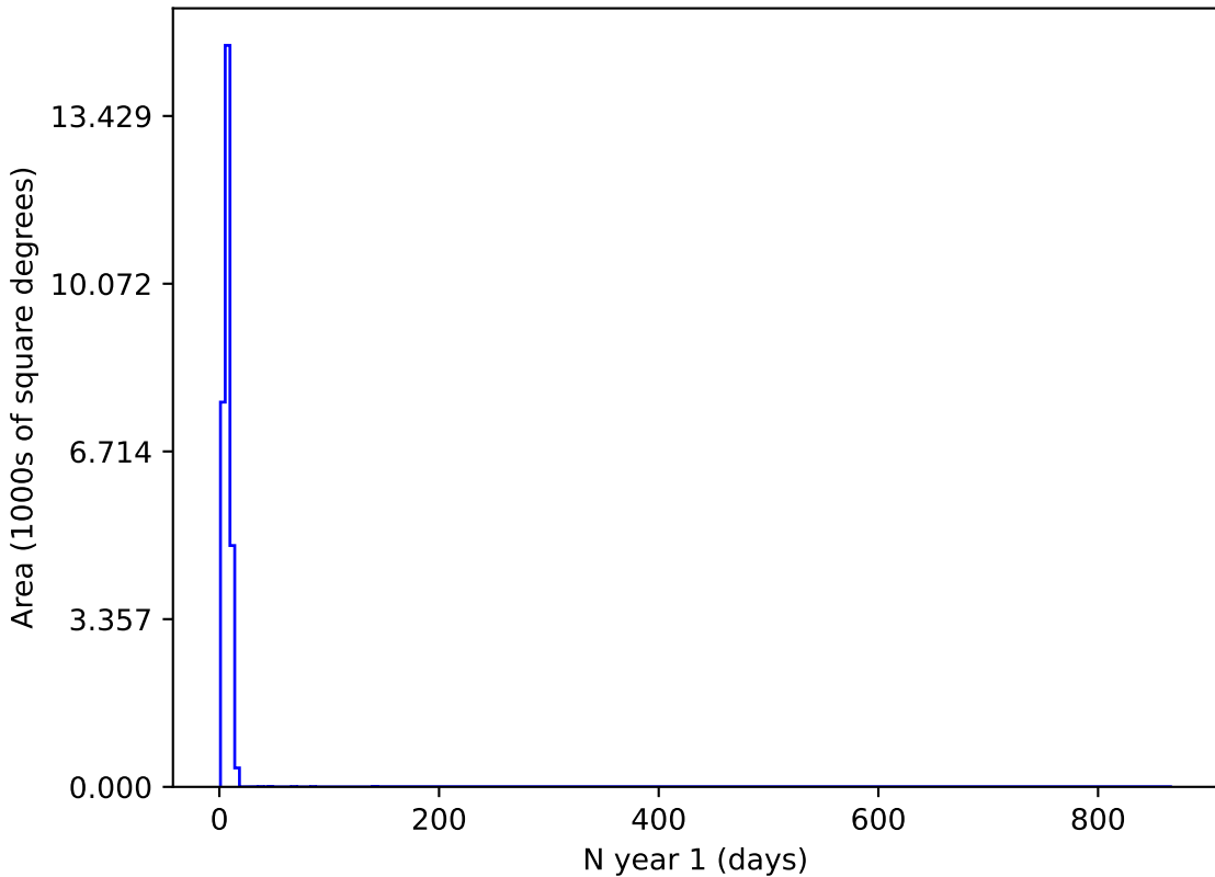
weather_cloudso0v3.4_10yrs g and night < 365: N year 1
