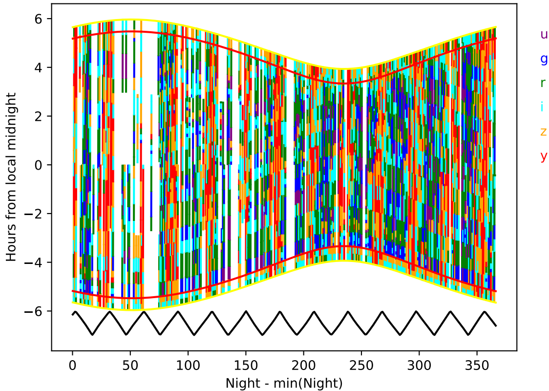
weather_cloudso0v3.4_10yrs year 9-10: Hourglass
