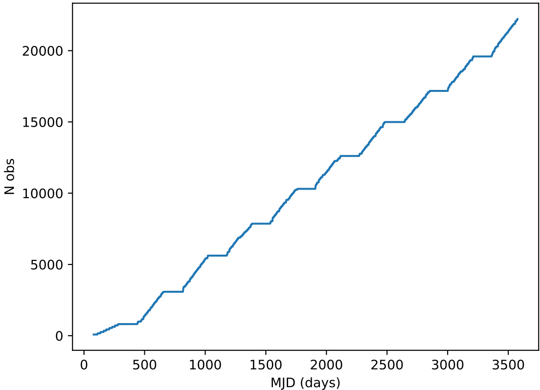
weather_cloudso0v3.4_10yrs note like DD:XMM_LSS%: Cumulative
