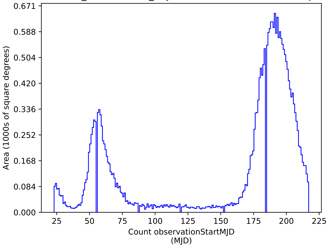
weather_cloudso0v3.4_10yrs i: Count observationStartMJD
