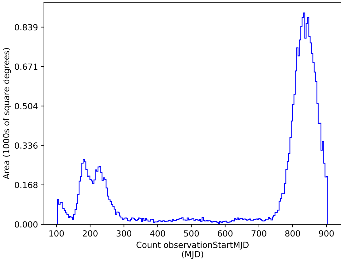
weather_cloudso0v3.4_10yrs : Count observationStartMJD
