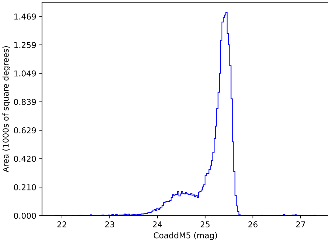
weather_cloudso0v3.4_10yrs u: CoaddM5
