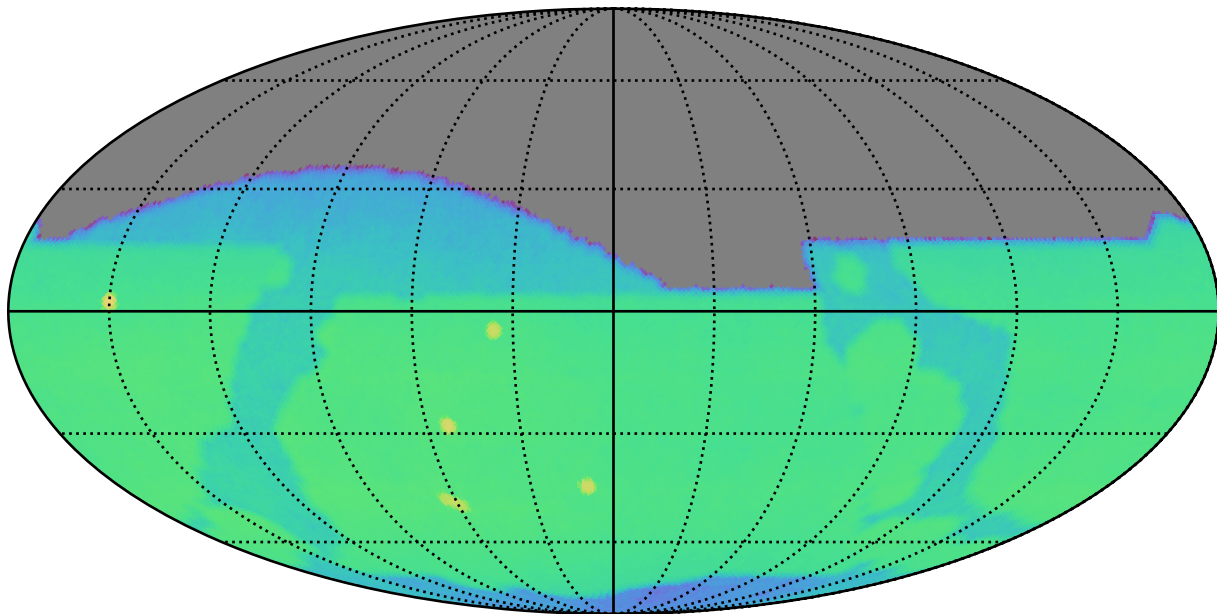
weather_cloudso0v3.4_10yrs r: CoaddM5
