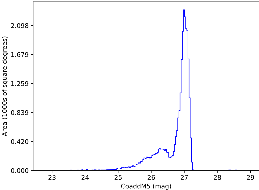
weather_cloudso0v3.4_10yrs r: CoaddM5
