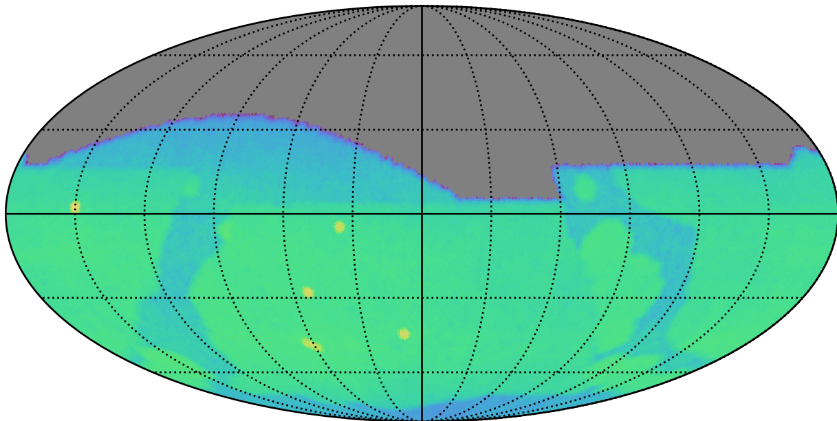
weather_cloudso0v3.4_10yrs g: CoaddM5
