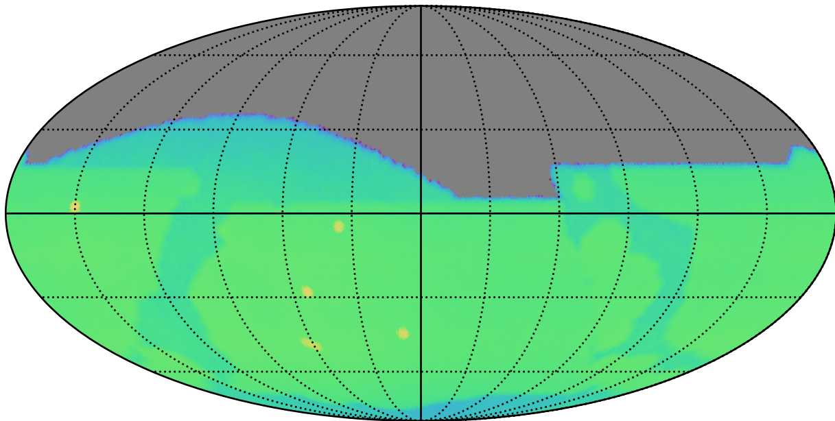
weather_cloudso0v3.4_10yrs : CoaddM5
