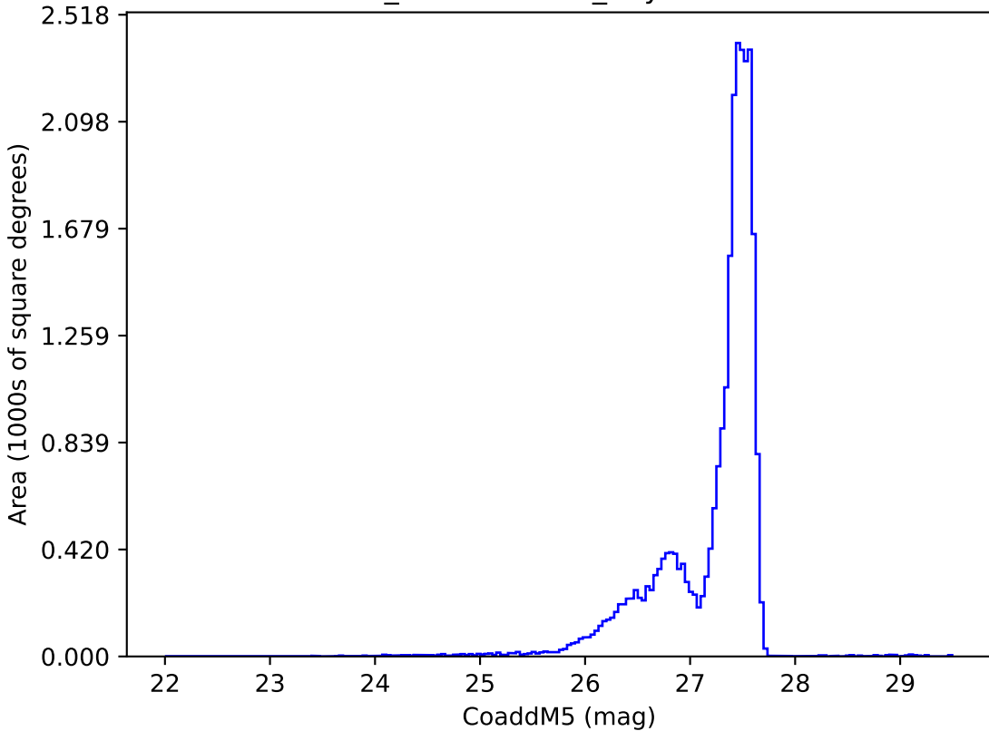
weather_cloudso0v3.4_10yrs : CoaddM5
