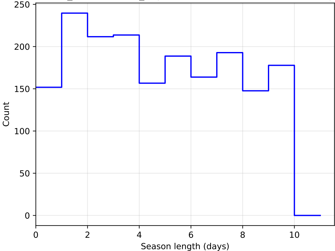
weather_cloudso0v3.4_10yrs DD:WFD all bands: SeasonLength
