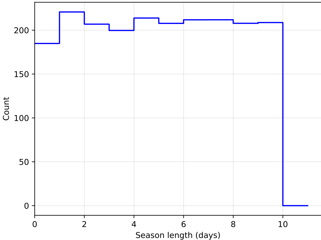
weather_cloudso0v3.4_10yrs DD:ELAISS1 all bands: SeasonLength
