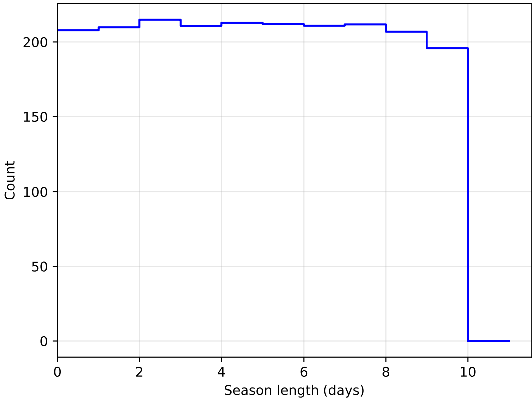
weather_cloudso0v3.4_10yrs DD:EDFS all bands: SeasonLength
