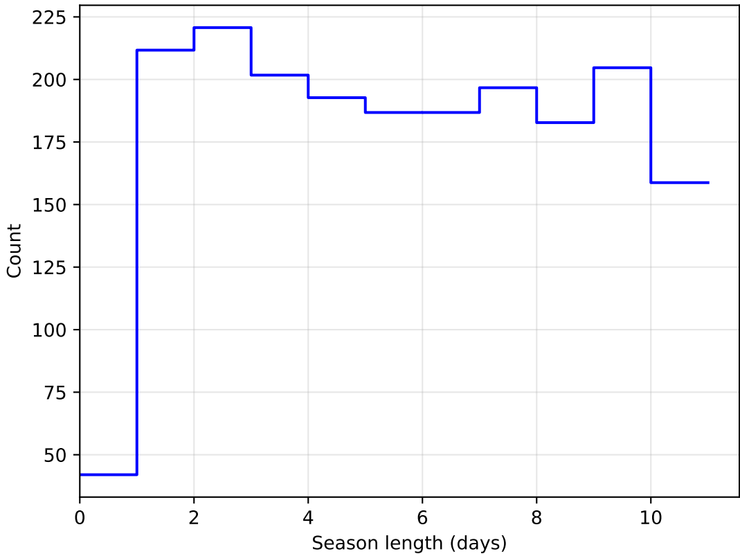
weather_cloudso0v3.4_10yrs DD: COSMOS all bands: SeasonLength
