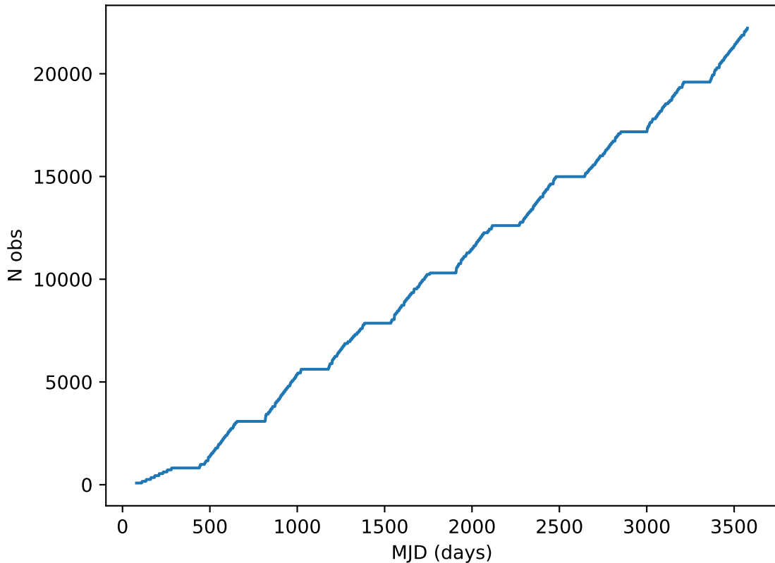
weather_cloudso0v3.4_10yrs all bands: DD:XMM_LSS Cumulative NVisits
