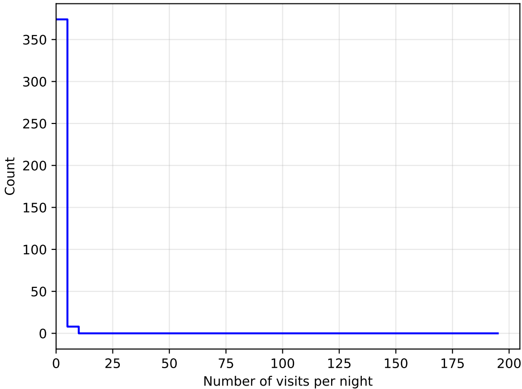
weather_cloudso0v3.4_10yrs all bands: DD:WFD NVisitsPerNight
