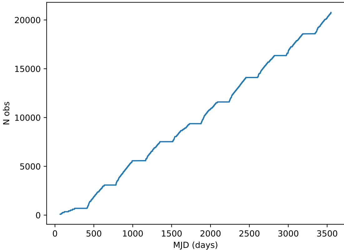
weather_cloudso0v3.4_10yrs all bands: DD:ELAISS1 Cumulative NVisits
