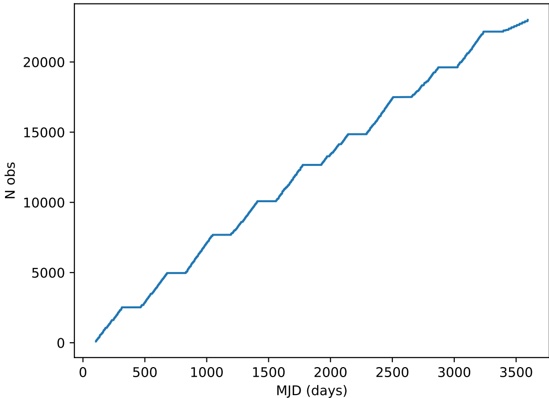
weather_cloudso0v3.4_10yrs all bands: DD:EDFS Cumulative NVisits
