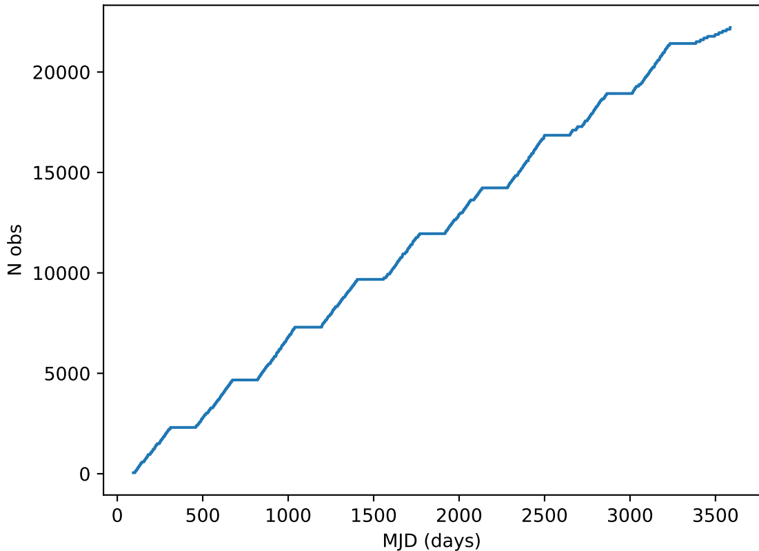
weather_cloudso0v3.4_10yrs all bands: DD:ECDFS Cumulative NVisits
