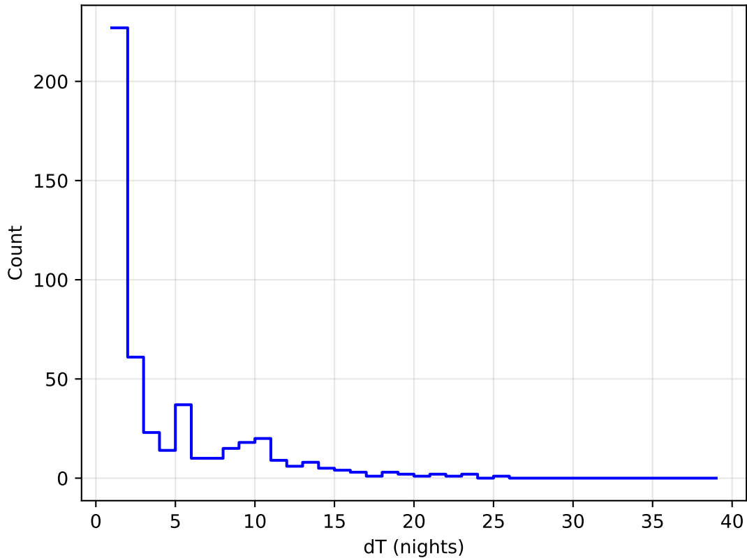
weather_cloudso0v3.4_10yrs all bands: DD: COSMOS Delta Nights Histogram
