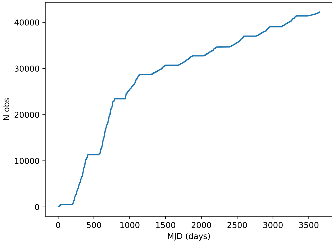
weather_cloudso0v3.4_10yrs all bands: DD:COSMOS Cumulative NVisits
