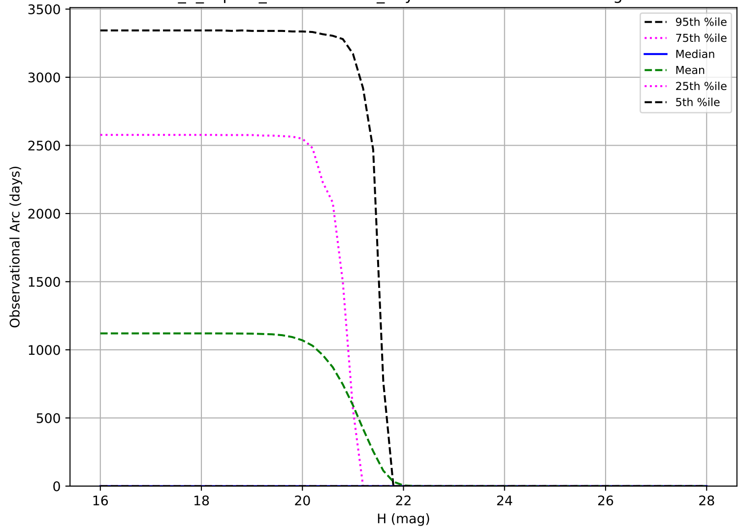
uniform_u_expt38_nscale1.1v3.4_10yrs: Observational Arc Length Vatra
