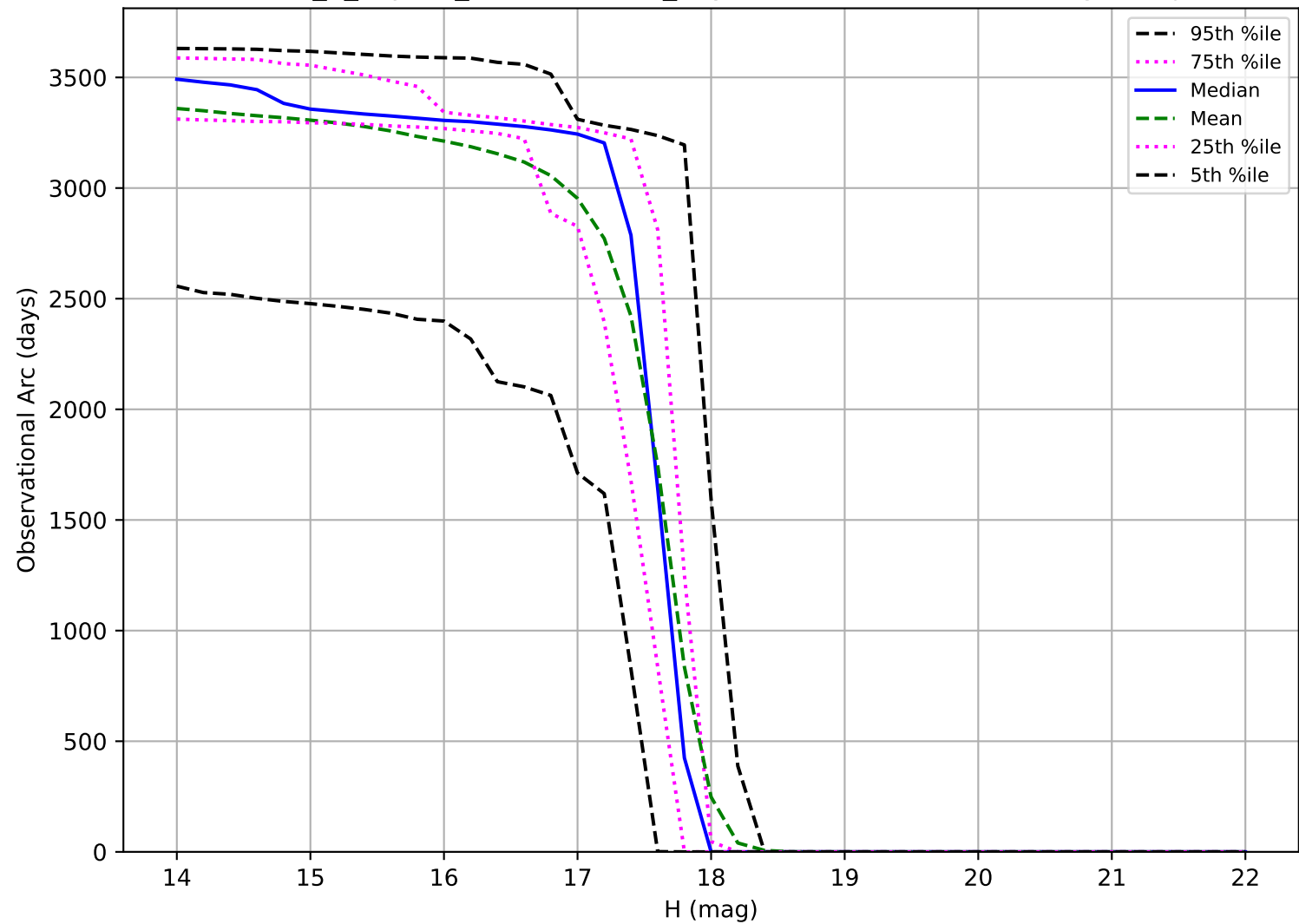
uniform_u_expt38_nscale1.1v3.4_10yrs: Observational Arc Length Trojan
