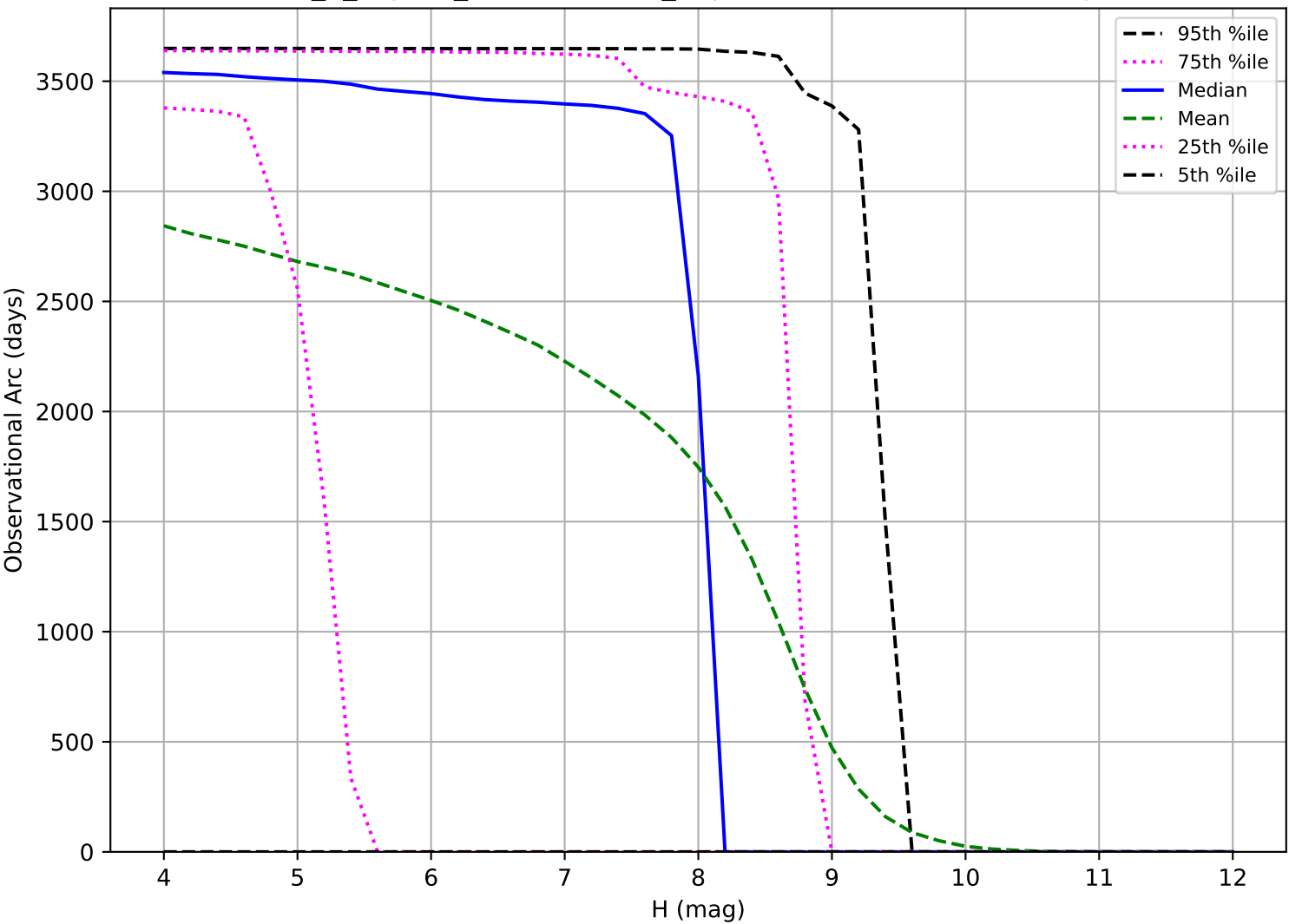
uniform_u_expt38_nscale1.1v3.4_10yrs: Observational Arc Length TNO
