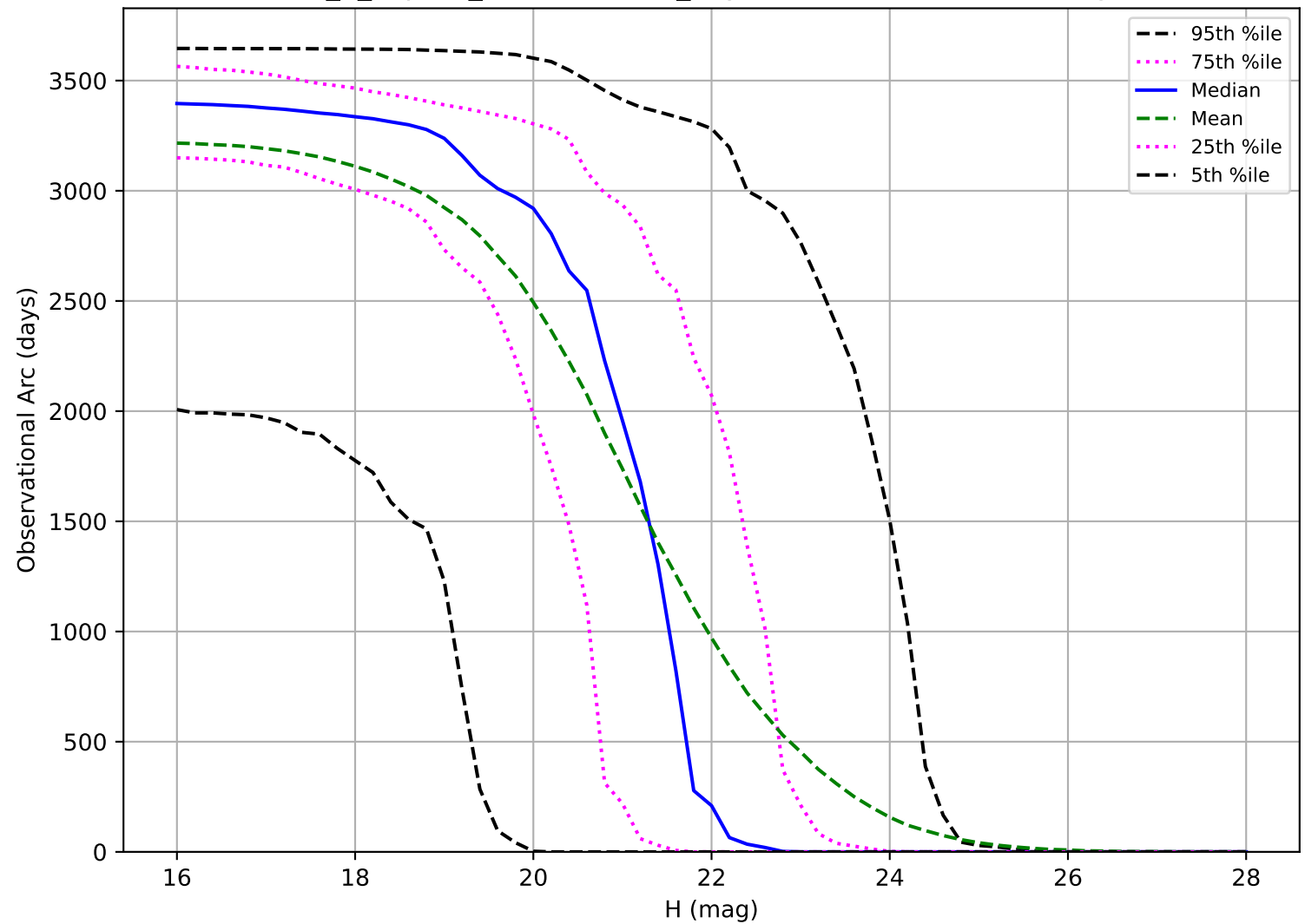
uniform_u_expt38_nscale1.1v3.4_10yrs: Observational Arc Length PHA
