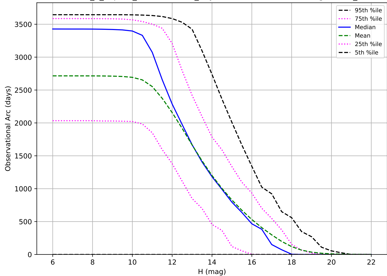
uniform_u_expt38_nscale1.1v3.4_10yrs: Observational Arc Length OCC_r5
